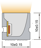
Unit: mm Cross section
